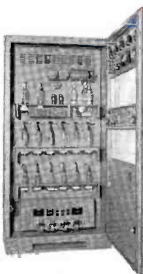
Front view of driver and rectifier cabinet, with covers removed. Vertical chassis design provides immediate access to all wiring and components, both front and rear.
